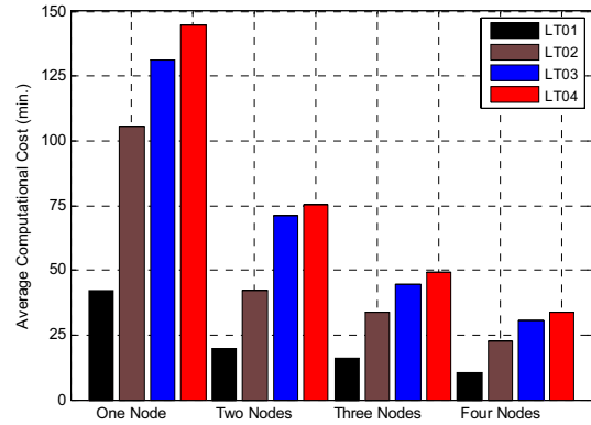
Figure 10. N-1-1 Contingency Analysis Computational Cost Comparisons
